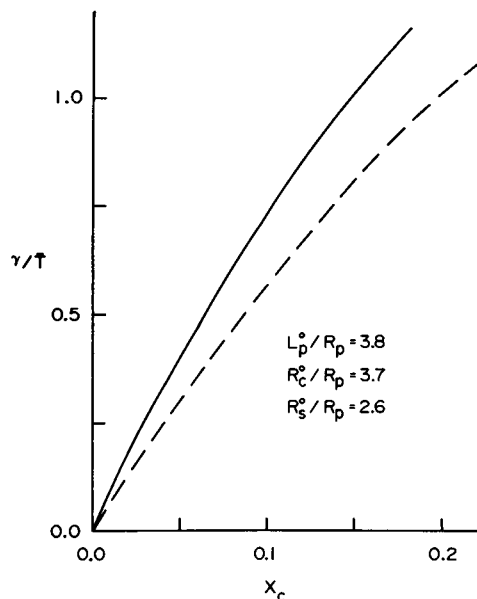
FIGURE 2 Sample computation of the free energy reduction per unit area of contact (affinity) normalized by the membrane tension for the following situations: the solid line represents the case where the pipettes maintain fixed positions which creates an axial force; the dashed curve represents the case where the pipettes are moved so that the vesicles maintain perfect spherical conformations during the adhesion process with no axial force. This specific example represents an initial geometry where the aspirated length of the adherent ( left ) vesicle is 3.8 pipette radii, the outer diameter of the adherent vesicle is 3.7 pipette radii, and the diameter of the rigid ( right ) vesicle is 2.6 pipette radii. The difference between the two curves is due to the presence of an axial force in the case where the pipettes are left at fixed positions.
